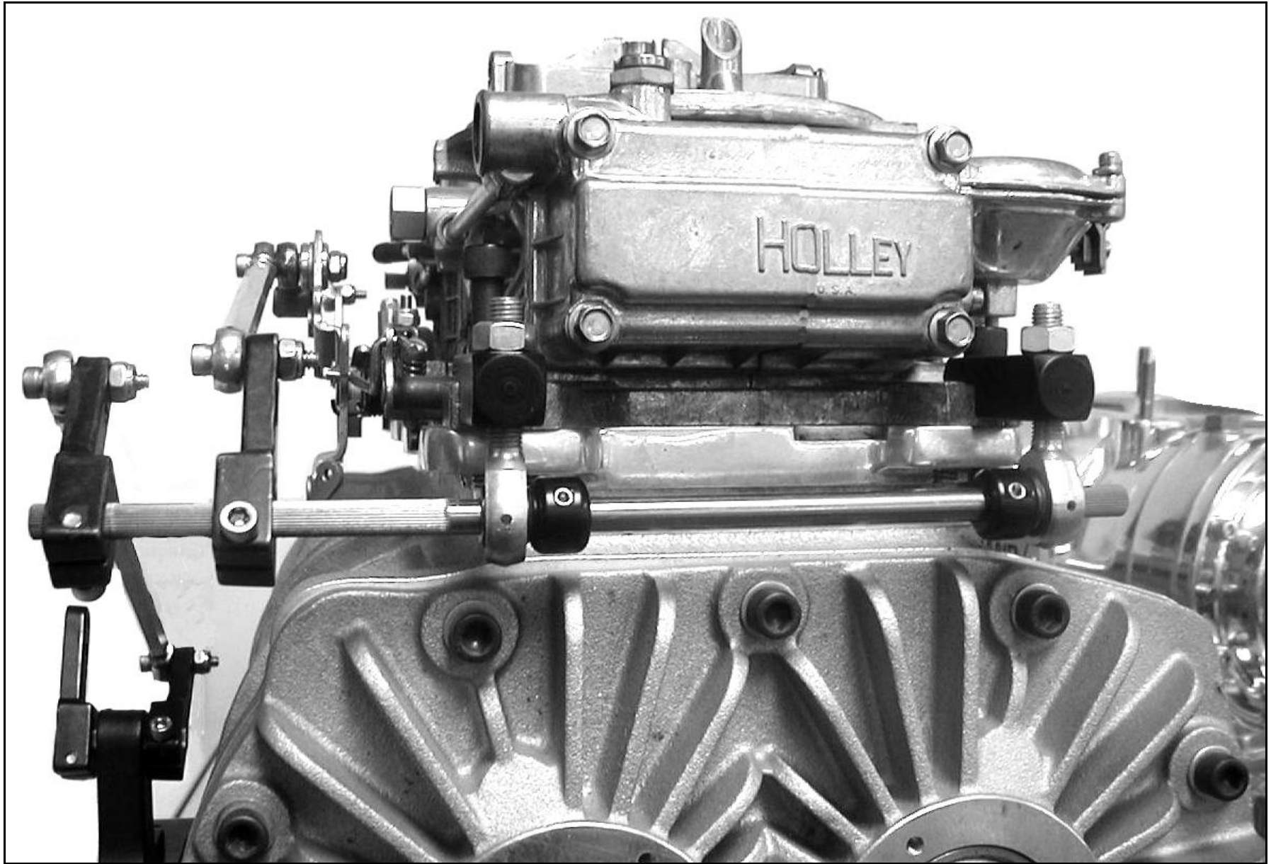
Side view of linkage kit
